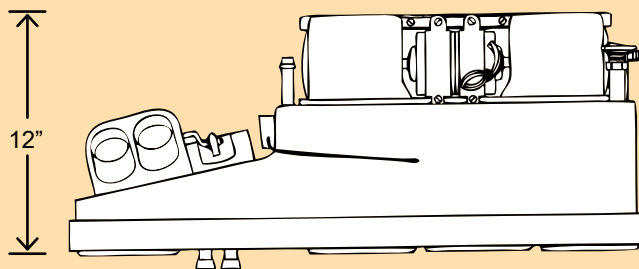
Slim Line Dimension Detail
